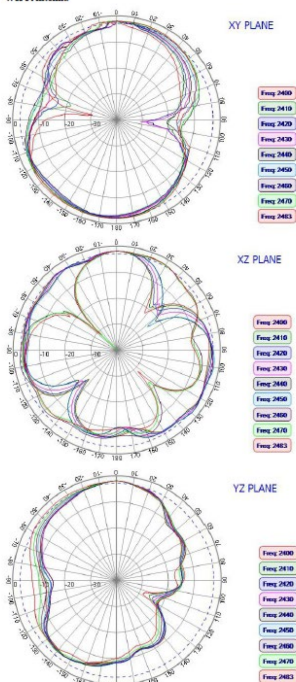
WIFI Antenna
